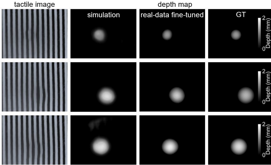
Fig. S12. Comparison of geometry reconstruction between simulation training and real-data fine-tuning.
